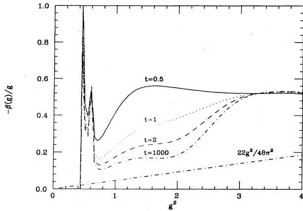
FIG. 9. Plot of a direct computation of the [2/4] \beta function by D -Padé approximating the series for -g/\beta(g) = g^2 d \log M^2 / dg^2 . Plots are given for t=0.5, 1, 2, 1000 .
