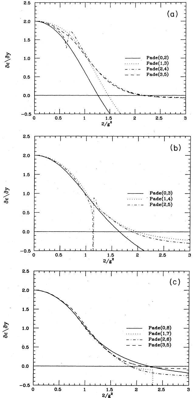
FIG. 1. Curves of d\mathcal{E}/dy obtained using the D -Padé technique. (a) d\mathcal{E}/dy computed by forming [L/(L+2)] -Padé approximants to \partial^2\mathcal{E}/\partial y\partial t . (b) [L/(L+3)] -Padé approximants to d^2\mathcal{E}/dydt . Note the pole in the [2/5] -Padé approximant. (c) Comparison of all [L/(8-L)] -Padé approximants in order to show that the different sets of approximants behave similarly when computed to the same order in t .
